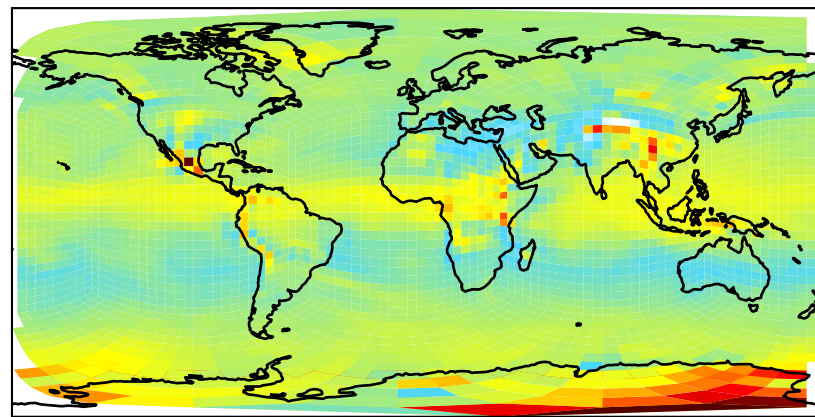
gchp-c24-1Mon-14.7.0-alpha.16 (Dev) c24
