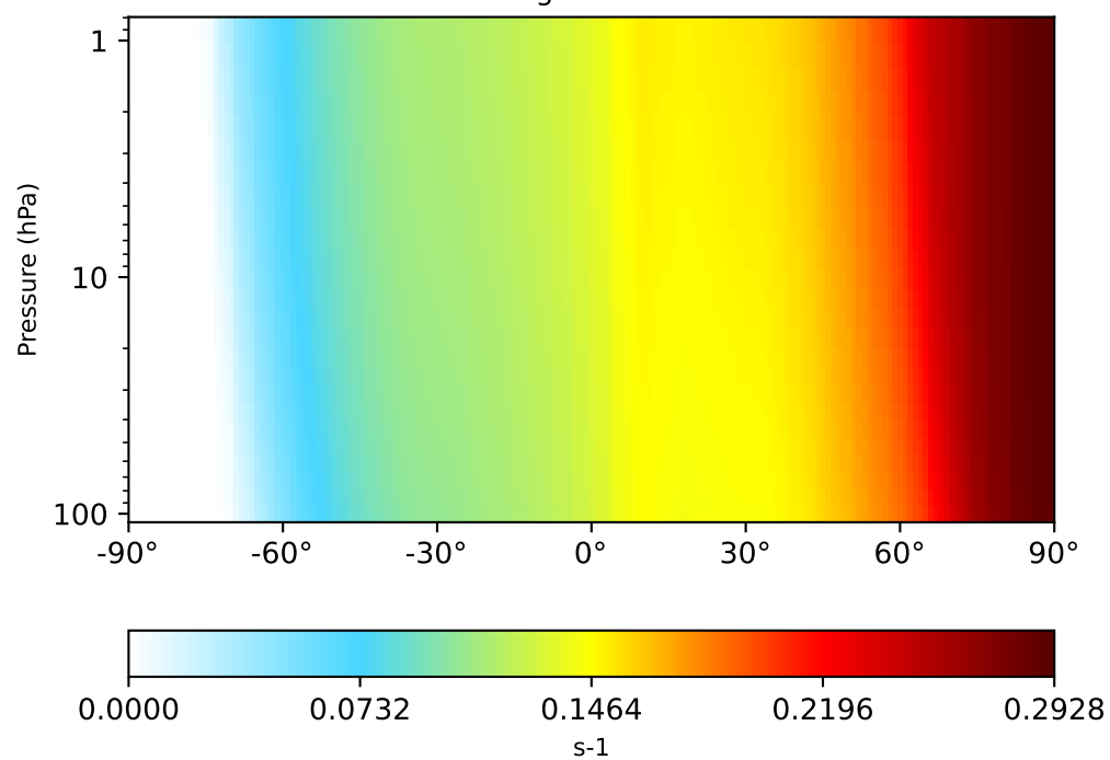
gchp-c24-1Mon-14.7.0-alpha.16 (Dev) 1x1.25 regrided from c24
