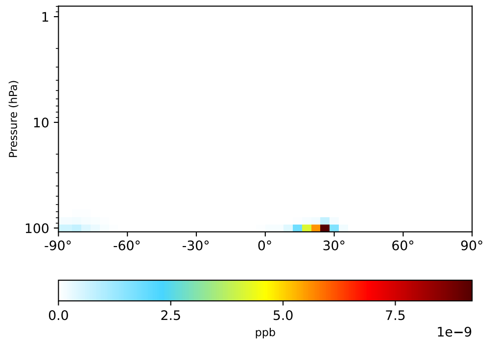
gcc-4x5-1Mon-14.7.0-alpha.17 (Dev) 4.0x5.0
