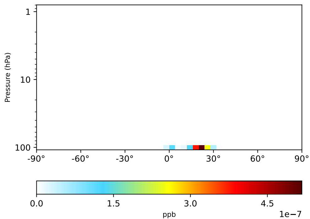
gcc-4x5-1Mon-14.7.0-alpha.16 (Ref) 4.0x5.0
