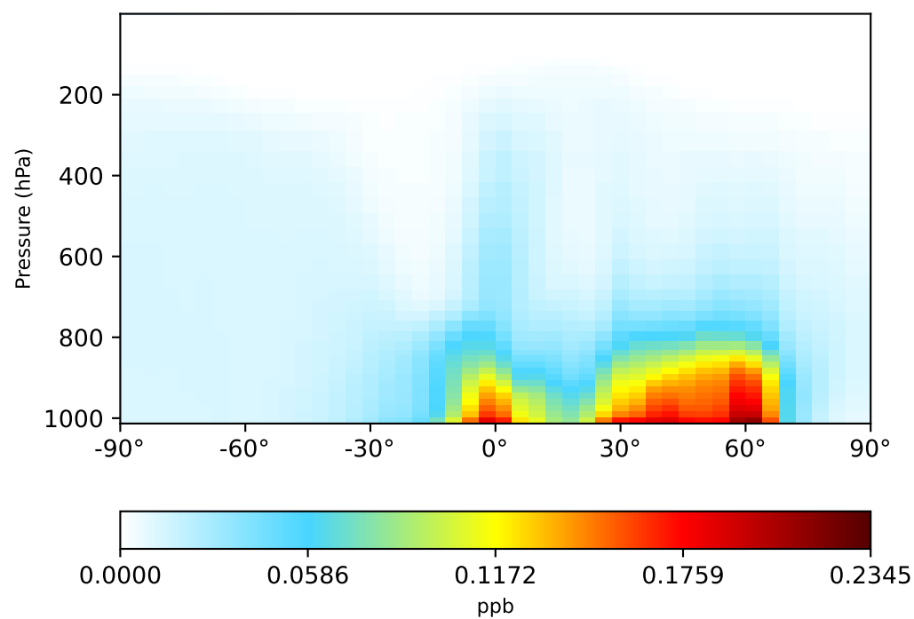
gcc-4x5-1Mon-14.7.0-alpha.15 (Ref) 4.0x5.0
