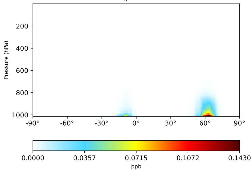
gchp-c24-1Mon-14.7.0-alpha.15 (Dev) 1x1.25 regridded from c24
