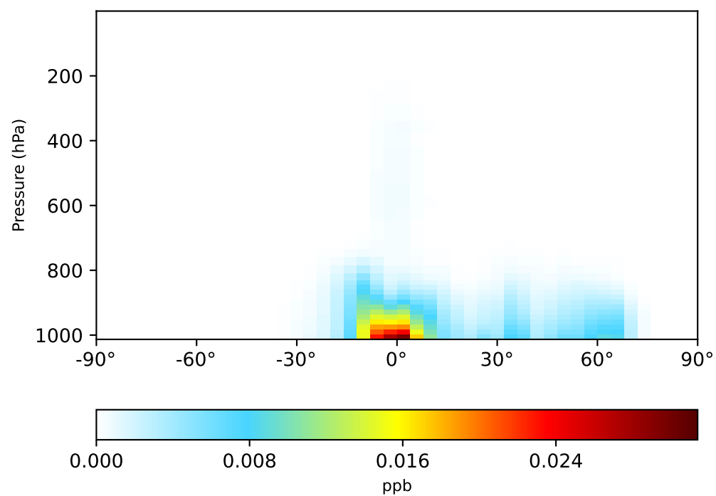
gcc-4x5-1Mon-14.7.0-alpha.15 (Ref) 4.0x5.0
