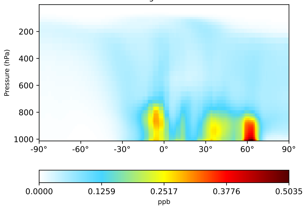
gchp-c24-1Mon-14.7.0-alpha.15 (Dev) 1x1.25 regrided from c24
