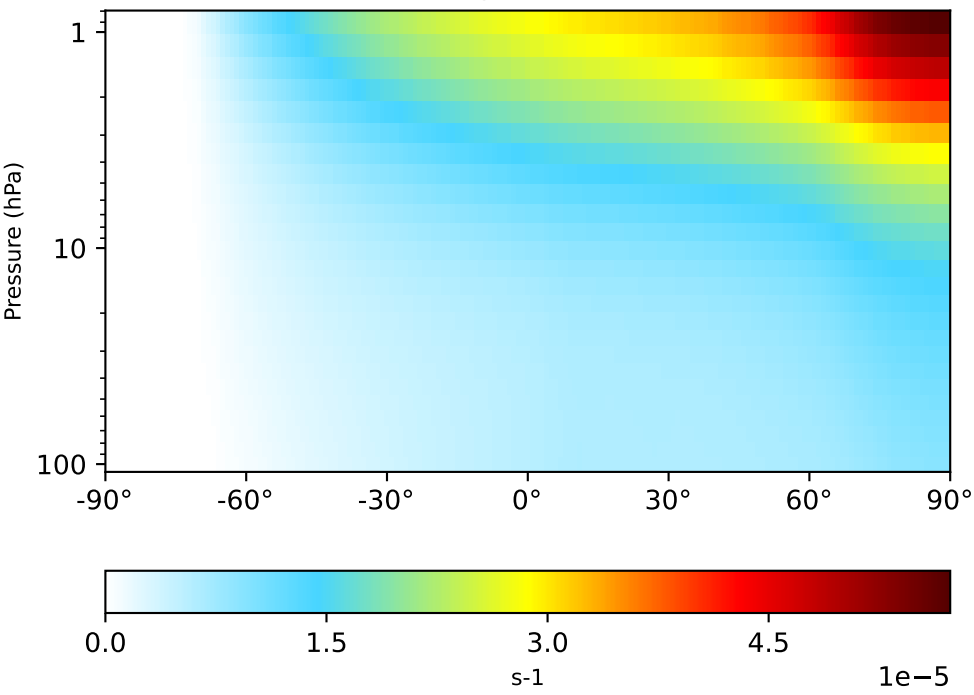
gchp-c24-1Mon-14.7.0-alpha.15 (Dev) 1x1.25 regridded from c24
