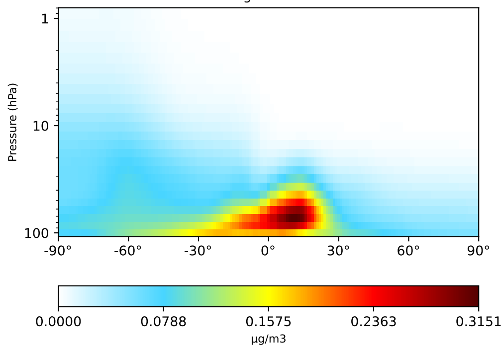
gchp-c24-1Mon-14.7.0-alpha.15 (Dev) 1x1.25 regrided from c24
