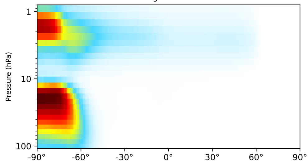
gchp-c24-1Mon-14.7.0-alpha.13 (Dev) 1x1.25 regridded from c24
