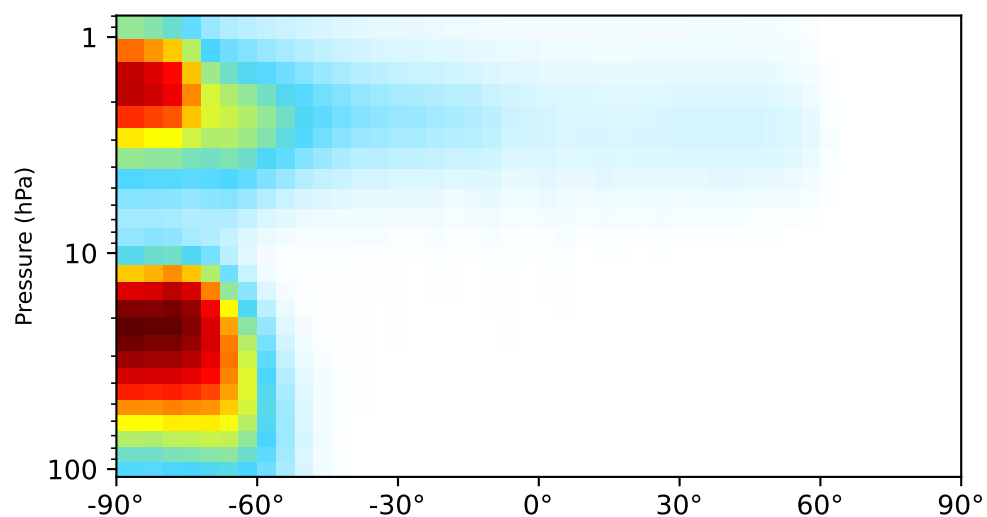
gcc-4x5-1Mon-14.7.0-alpha.13 (Ref) 4.0x5.0
