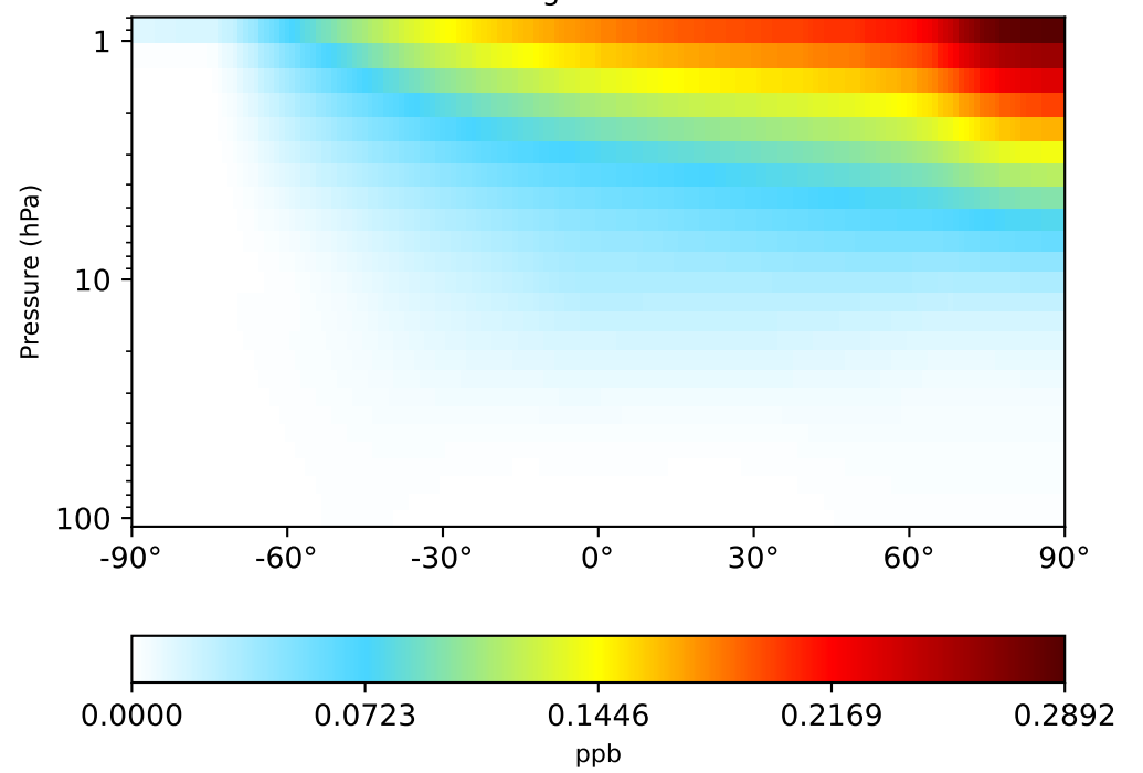
gchp-c24-1Mon-14.7.0-alpha.12 (Dev) 1x1.25 regrided from c24
