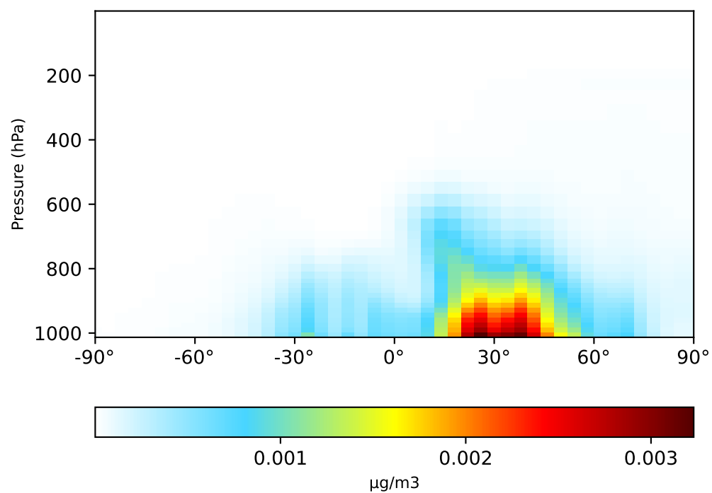
gcc-4x5-1Mon-14.7.0-alpha.13 (Dev) 4.0x5.0
