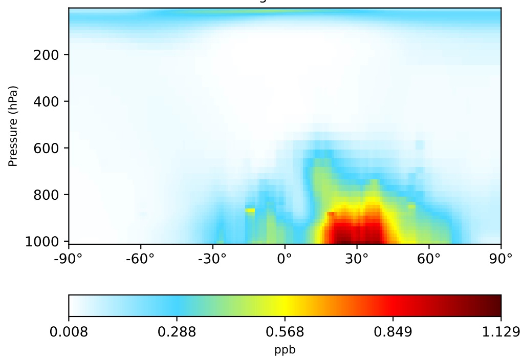
gchp-c24-1Mon-14.7.0-alpha.11 (Dev) 1x1.25 regrided from c24
