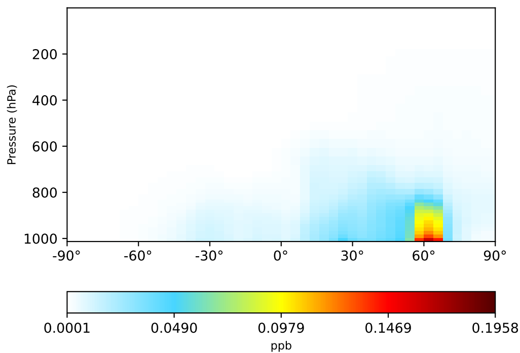
gcc-4x5-1Mon-14.7.0-alpha.11 (Ref) 4.0x5.0
