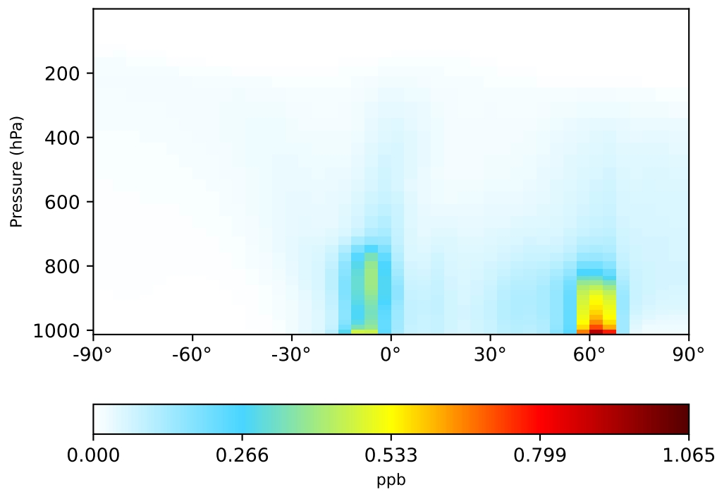
gcc-4x5-1Mon-14.7.0-alpha.11 (Ref) 4.0x5.0
