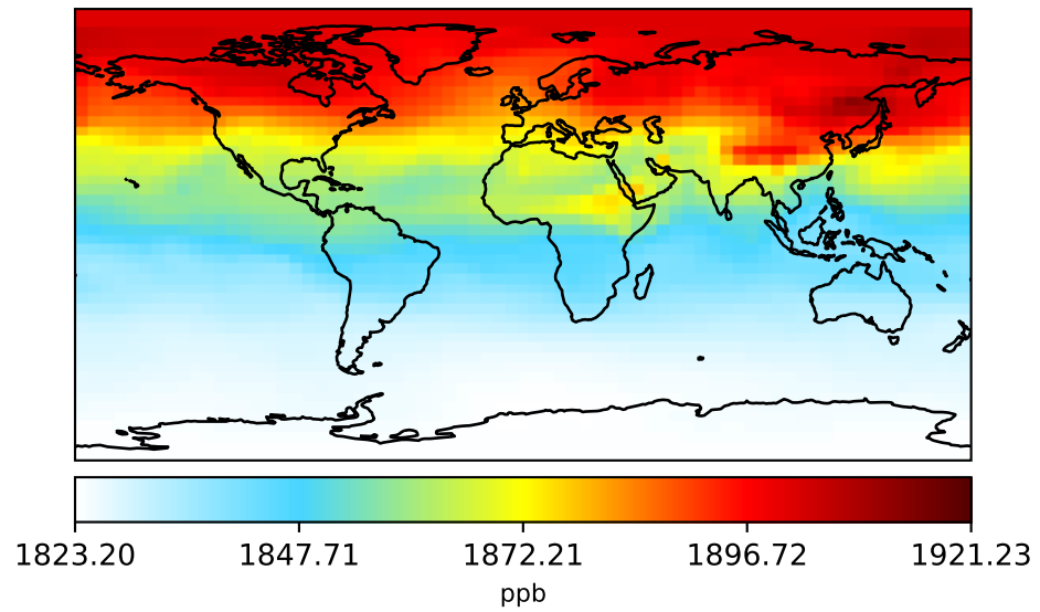
gcc-4x5-1Mon-14.7.0-alpha.11 (Ref) 4.0x5.0
