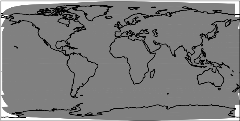
gchp-c24-1Mon-14.7.0-alpha.11 (Dev) c24
