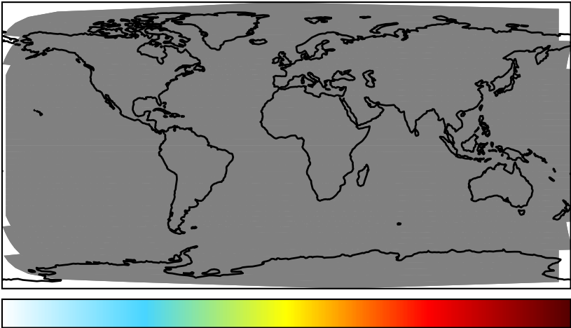
Undefined throughout domain s-1
