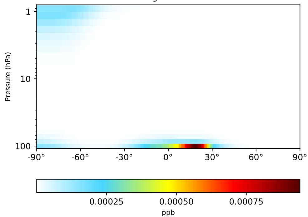
gchp-c24-1Mon-14.7.0-alpha.10 (Dev) 1x1.25 regrided from c24
