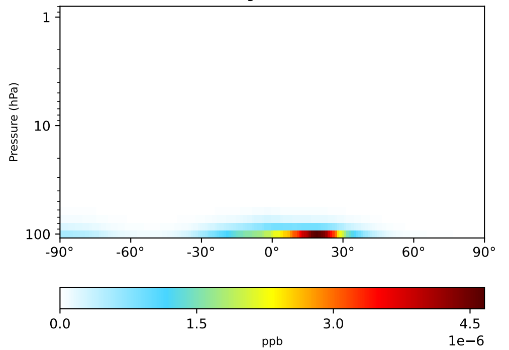
gchp-c24-1Mon-14.7.0-alpha.10 (Dev) 1x1.25 regrided from c24
