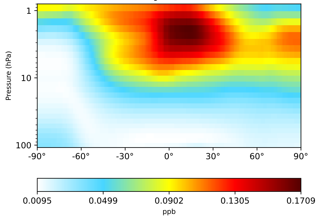
gchp-c24-1Mon-14.7.0-alpha.10 (Dev) 1x1.25 regrided from c24
