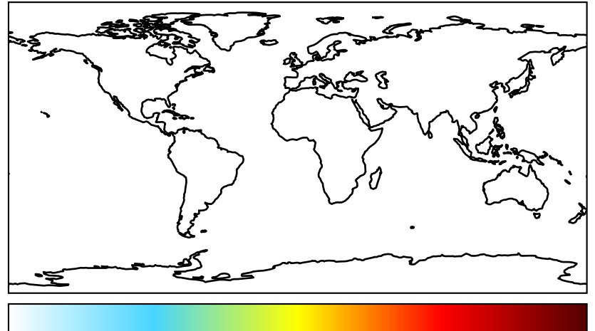
gchp-c24-1Mon-14.7.0-alpha.10 (Dev) c24
