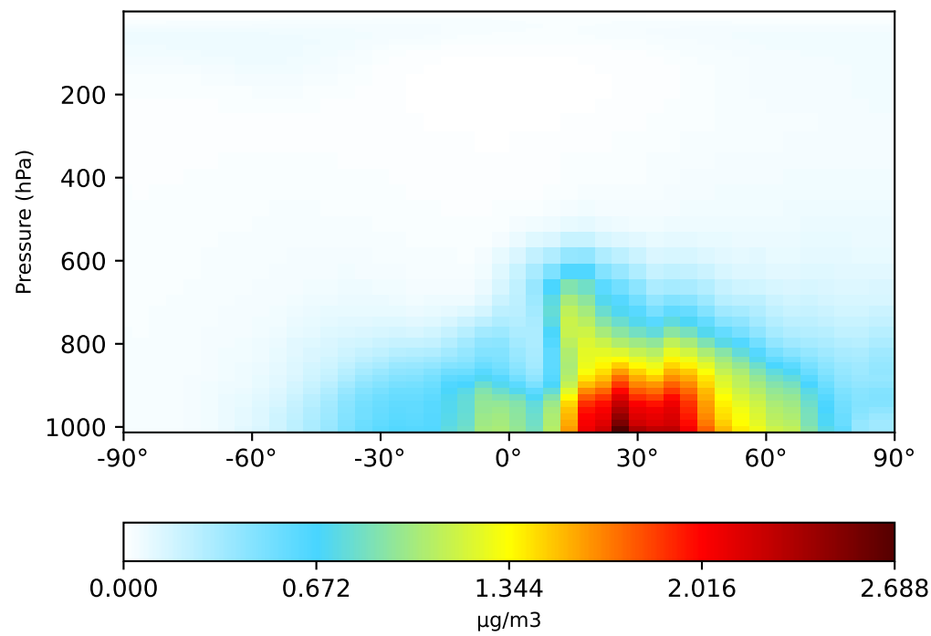
gcc-4x5-1Mon-14.7.0-alpha.10 (Ref) 4.0x5.0
