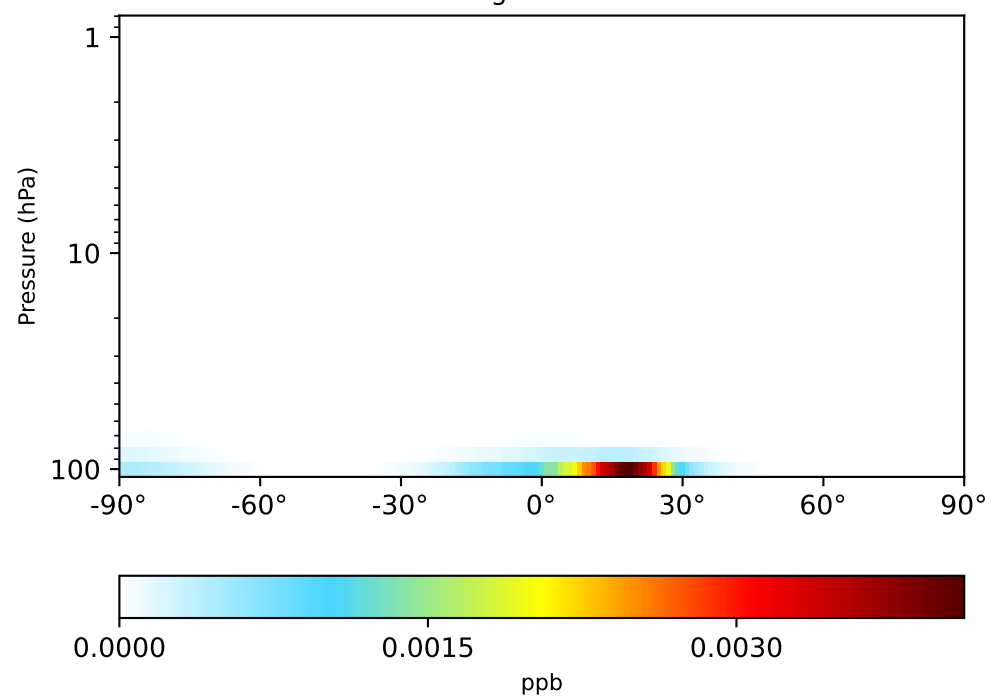
gchp-c24-1Mon-14.7.0-alpha.1 (Dev) 1x1.25 regrided from c24
