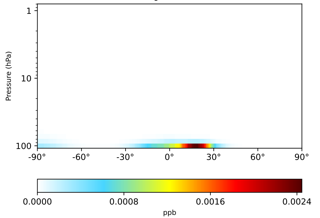
gchp-c24-1Mon-14.7.0-alpha.1 (Dev) 1x1.25 regrided from c24
