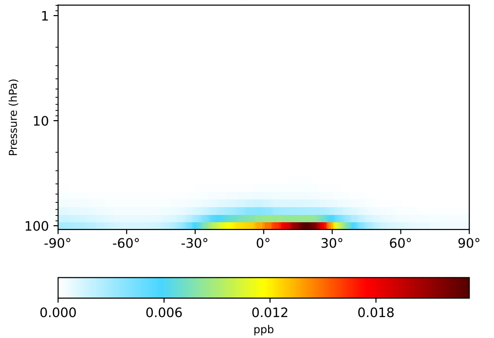
gchp-c24-1Mon-14.7.0-alpha.1 (Dev) 1x1.25 regrided from c24
