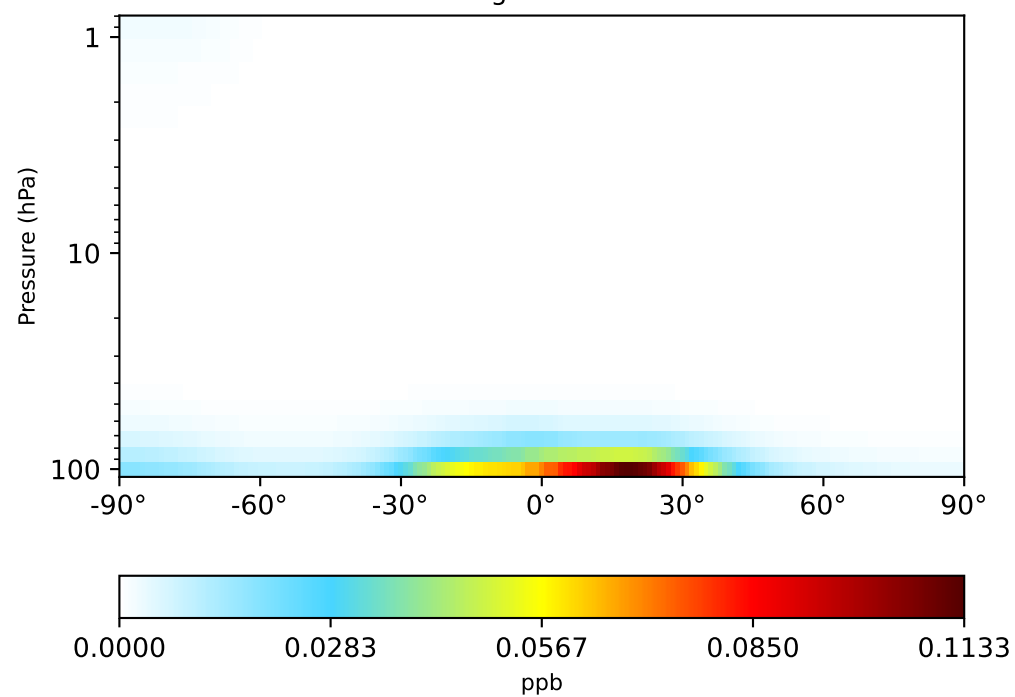
gchp-c24-1Mon-14.7.0-alpha.0 (Dev) 1x1.25 regrided from c24
