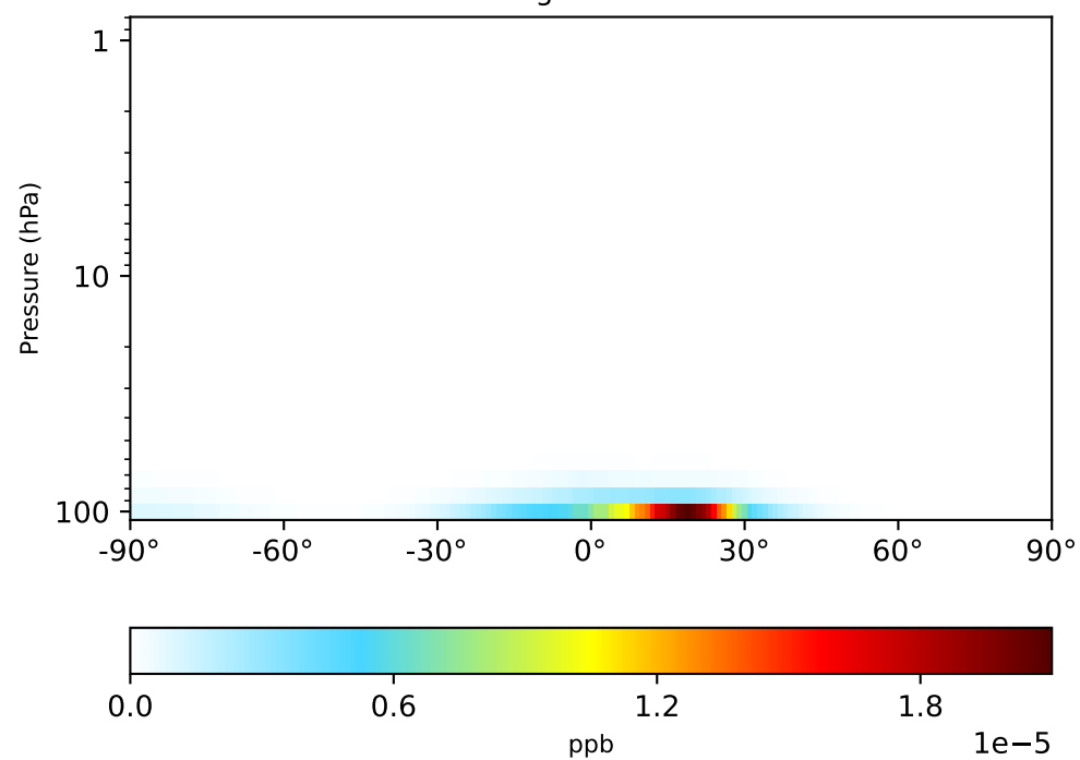
gchp-c24-1Mon-14.7.0-alpha.0 (Dev) 1x1.25 regrided from c24
