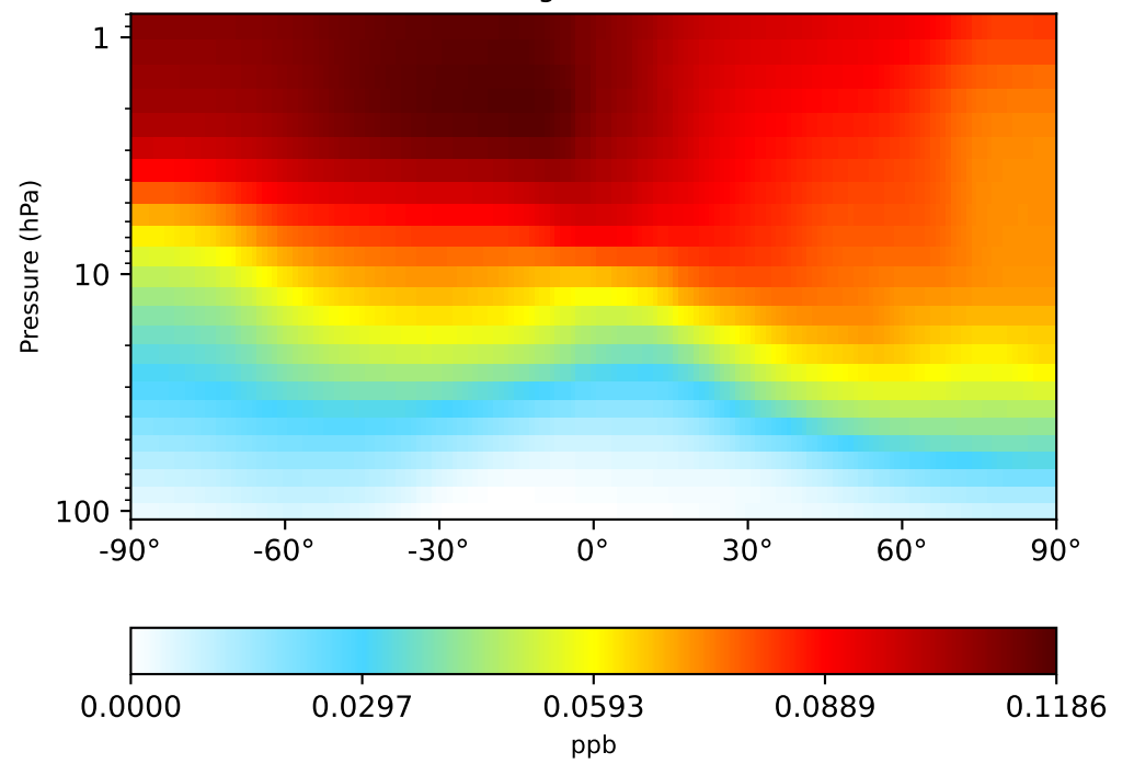
gchp-c24-1Mon-14.7.0-alpha.0 (Dev) 1x1.25 regrided from c24
