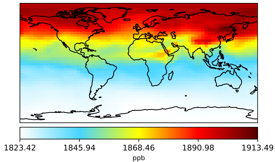
gcc-4x5-1Mon-14.6.3 (Ref) 4.0x5.0
