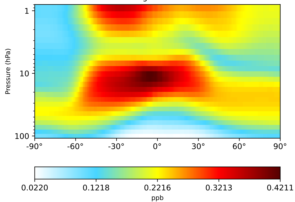
gchp-c24-1Mon-14.6.2 (Dev) 1x1.25 regrided from c24
