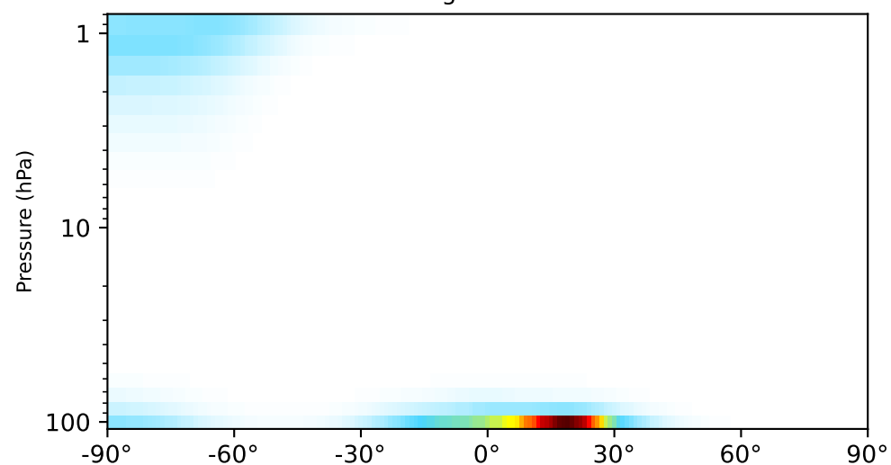
gchp-c24-1Mon-14.6.2 (Dev) 1x1.25 regrided from c24
