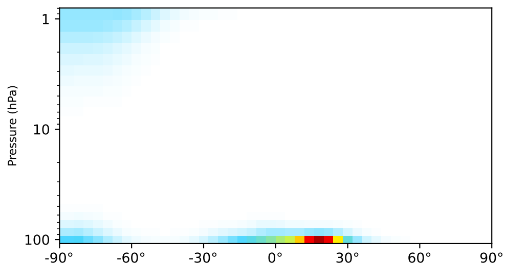
gcc-4x5-1Mon-14.6.2 (Ref) 4.0x5.0
