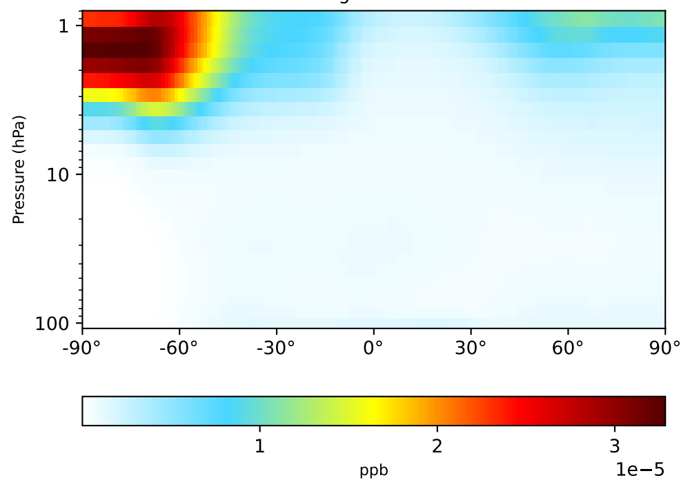
gchp-c24-1Mon-14.6.2 (Dev) 1x1.25 regridded from c24
