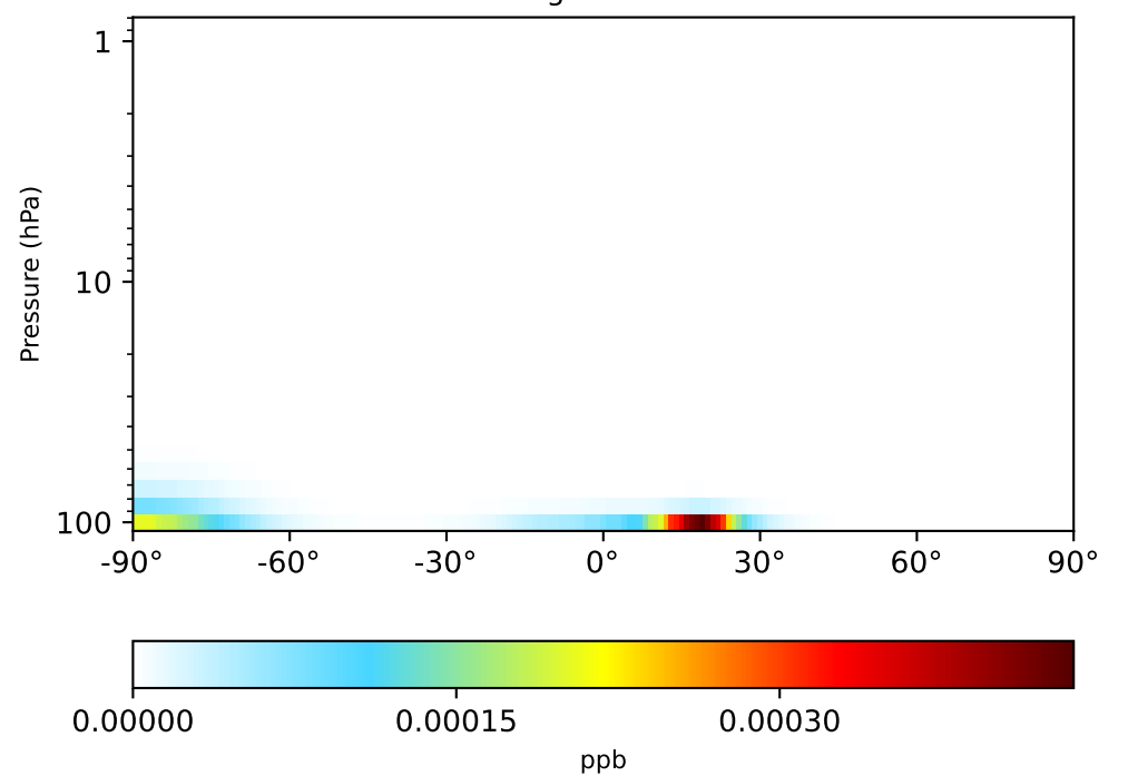
gchp-c24-1Mon-14.6.0-alpha.1 (Dev) 1x1.25 regrided from c24
