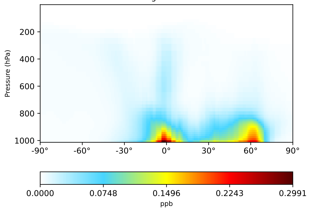
gchp-c24-1Mon-14.6.0-alpha.1 (Dev) 1x1.25 regrided from c24
