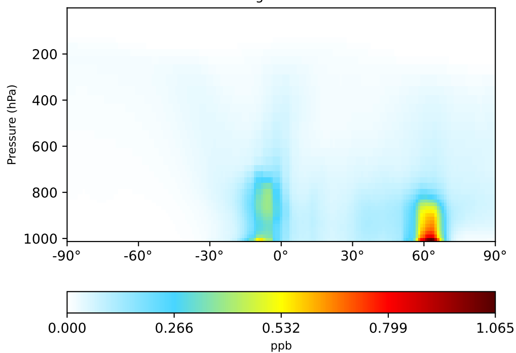
gchp-c24-1Mon-14.5.0-alpha.2 (Dev) 1x1.25 regridded from c24
