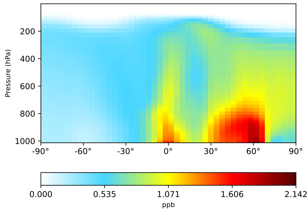
gcc-4x5-1Mon-14.5.0-alpha.2 (Ref) 4.0x5.0
