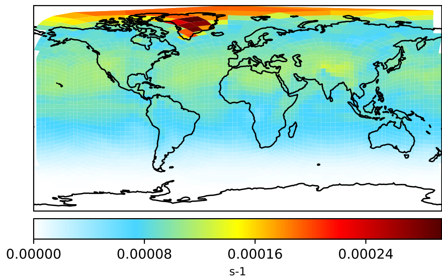
gchp-c24-1Mon-14.5.0-alpha.2 (Dev) c24
