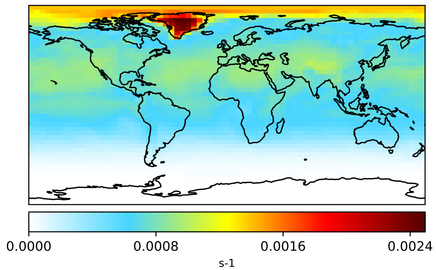
gcc-4x5-1Mon-14.5.0-alpha.2 (Ref) 4.0x5.0
