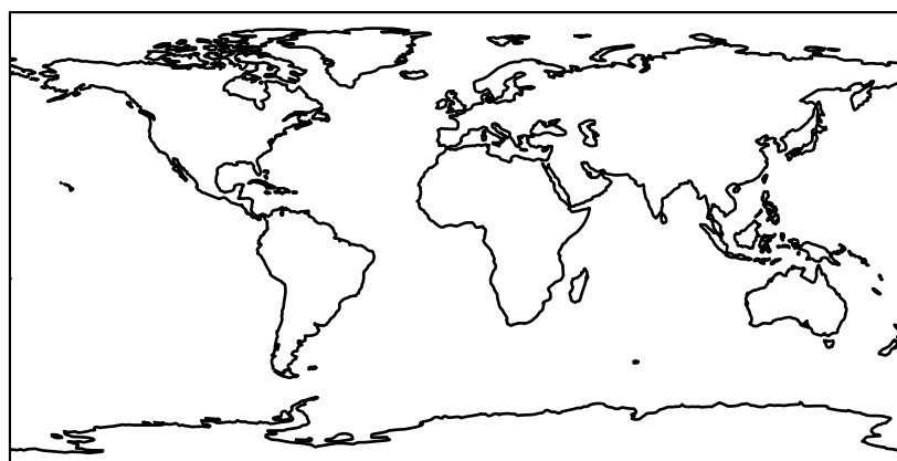
gchp-c24-1Mon-14.5.0-alpha.2 (Dev) c24
