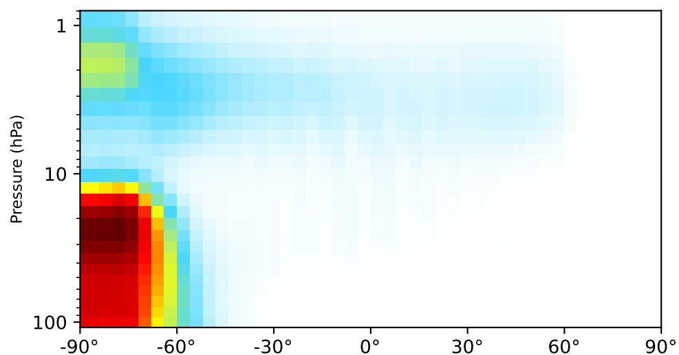
gcc-4x5-1Mon-14.5.0-alpha.2 (Ref) 4.0x5.0
