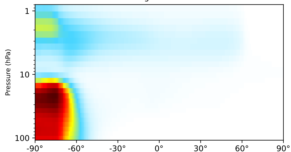
gchp-c24-1Mon-14.5.0-alpha.2 (Dev) 1x1.25 regridded from c24
