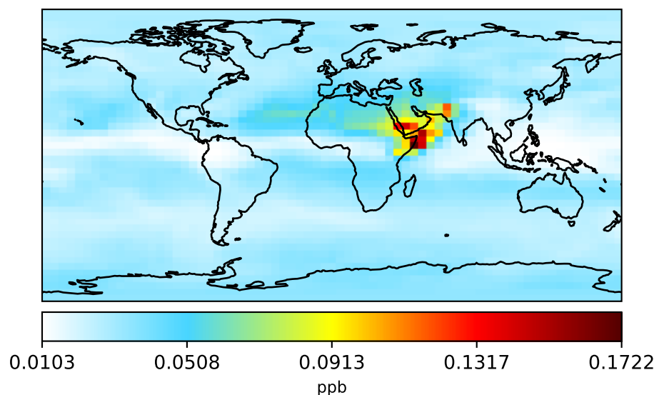
gcc-4x5-1Mon-14.5.0-alpha.2 (Ref) 4.0x5.0
