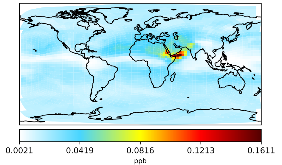
gchp-c24-1Mon-14.5.0-alpha.2 (Dev) c24
