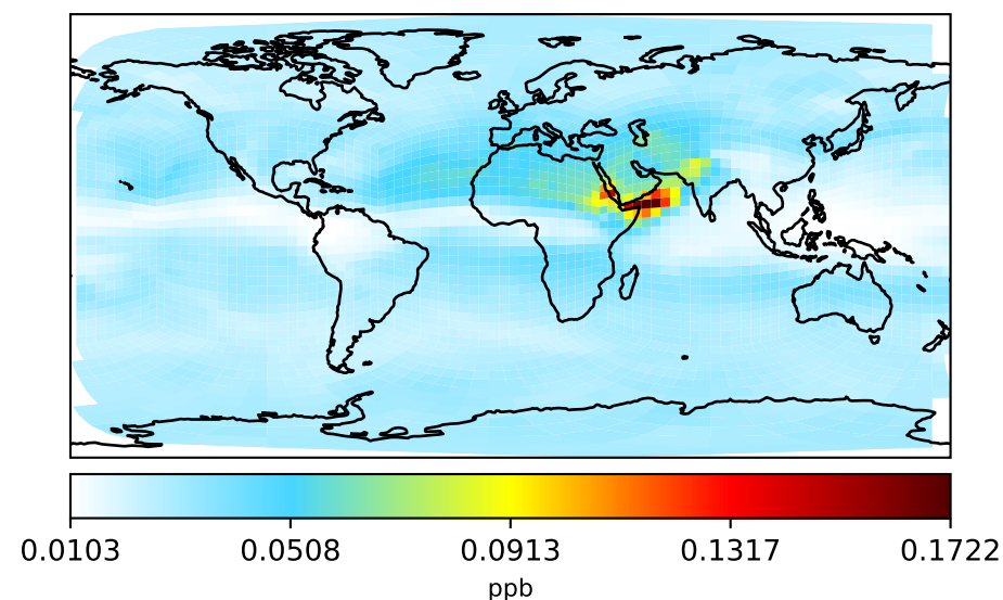
gchp-c24-1Mon-14.5.0-alpha.2 (Dev) c24
