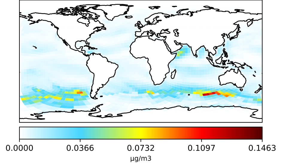
gchp-c24-1Mon-14.5.0-alpha.2 (Dev) c24
