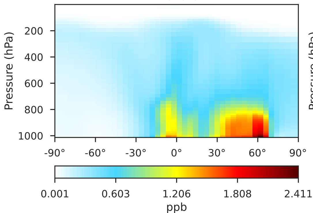
gcc-4x5-1Mon-14.2.2 (Ref) 4.0x5.0
