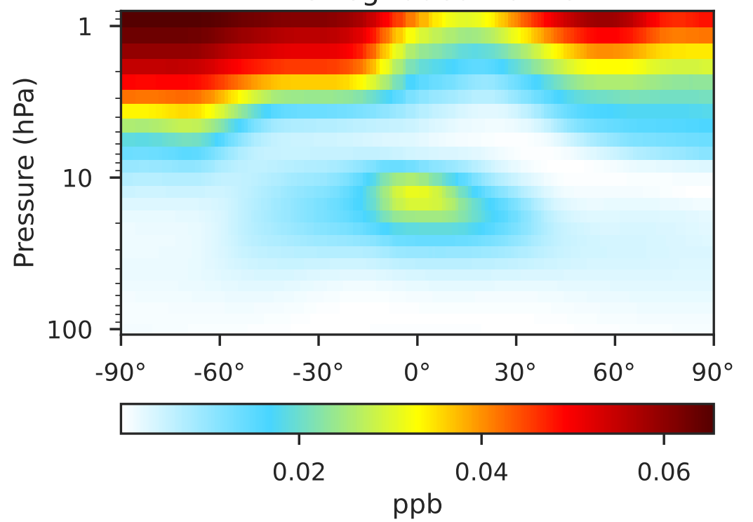
gchp-c24-1Mon-14.2.0-alpha.20 (Dev) 1x1.25 regridded from c24
