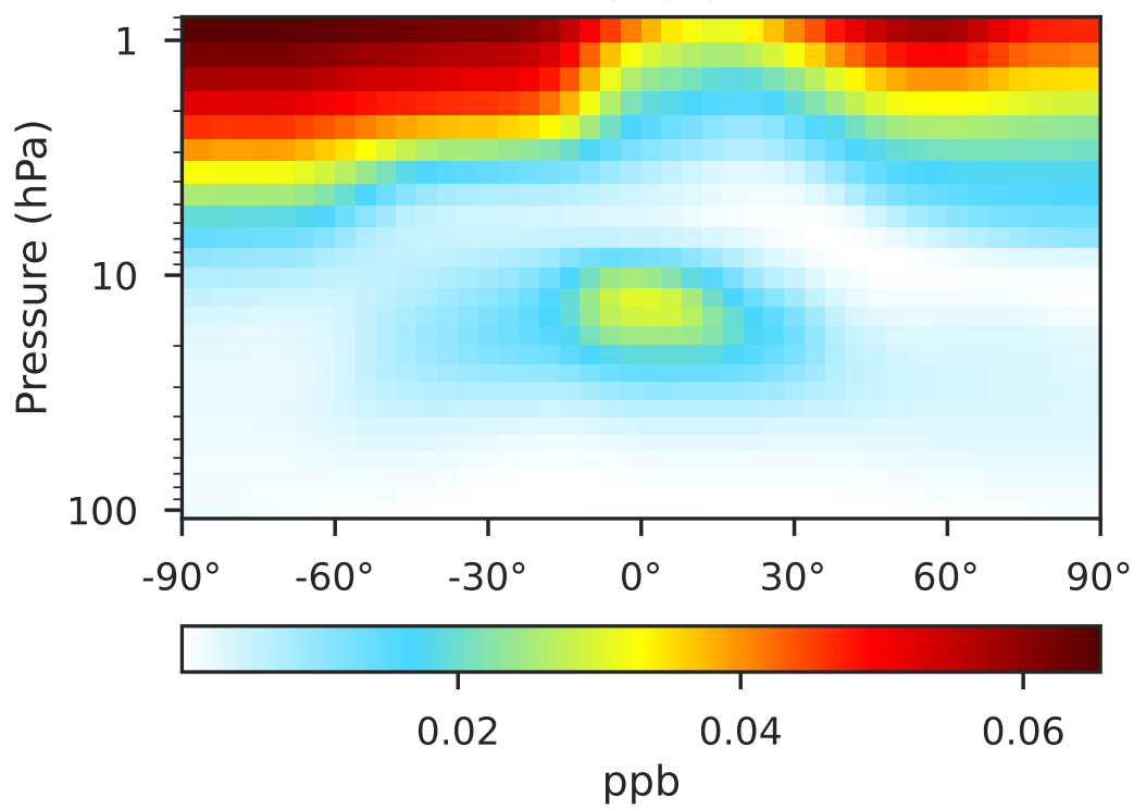
gcc-4x5-1Mon-14.2.0-alpha.20 (Ref) 4.0x5.0
