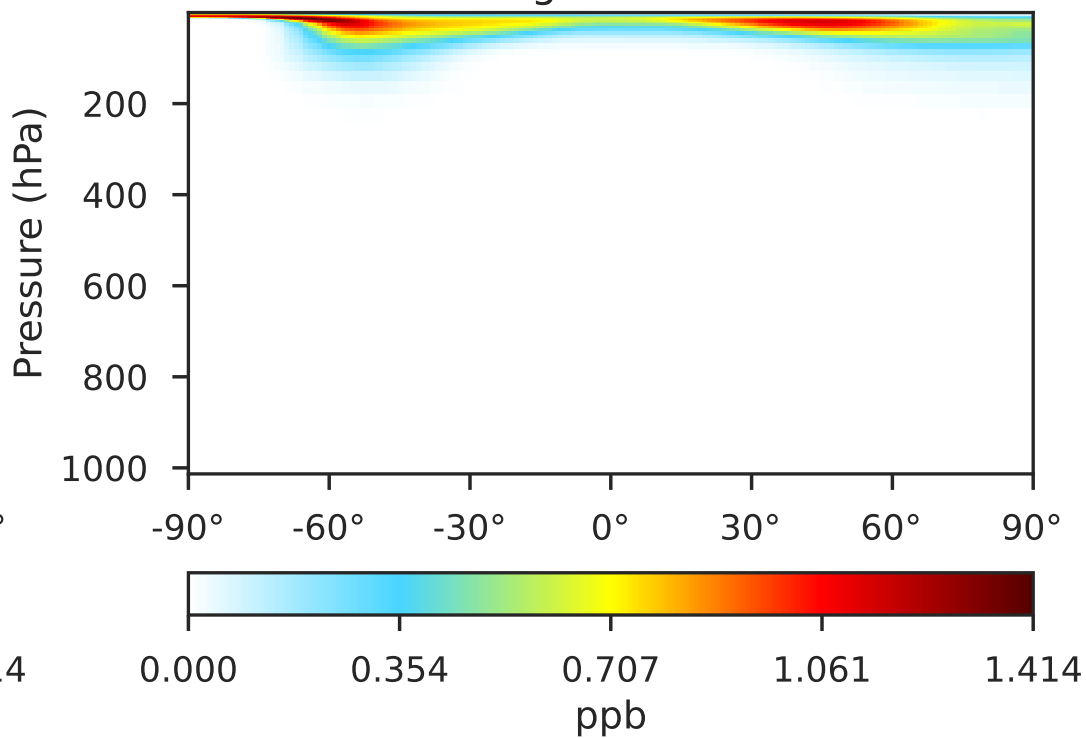
gchp-c24-1Mon-14.2.0-alpha.20 (Dev) 1x1.25 regridded from c24
