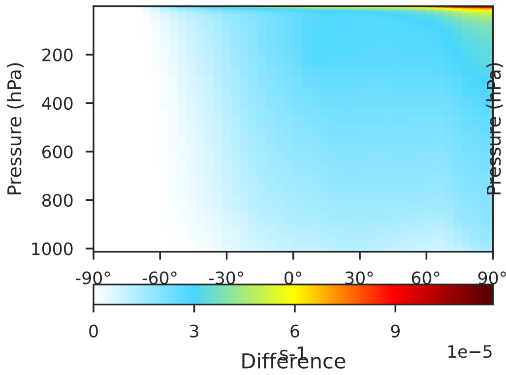
gcc-4x5-1Mon-14.1.1 (Ref) 4.0x5.0
