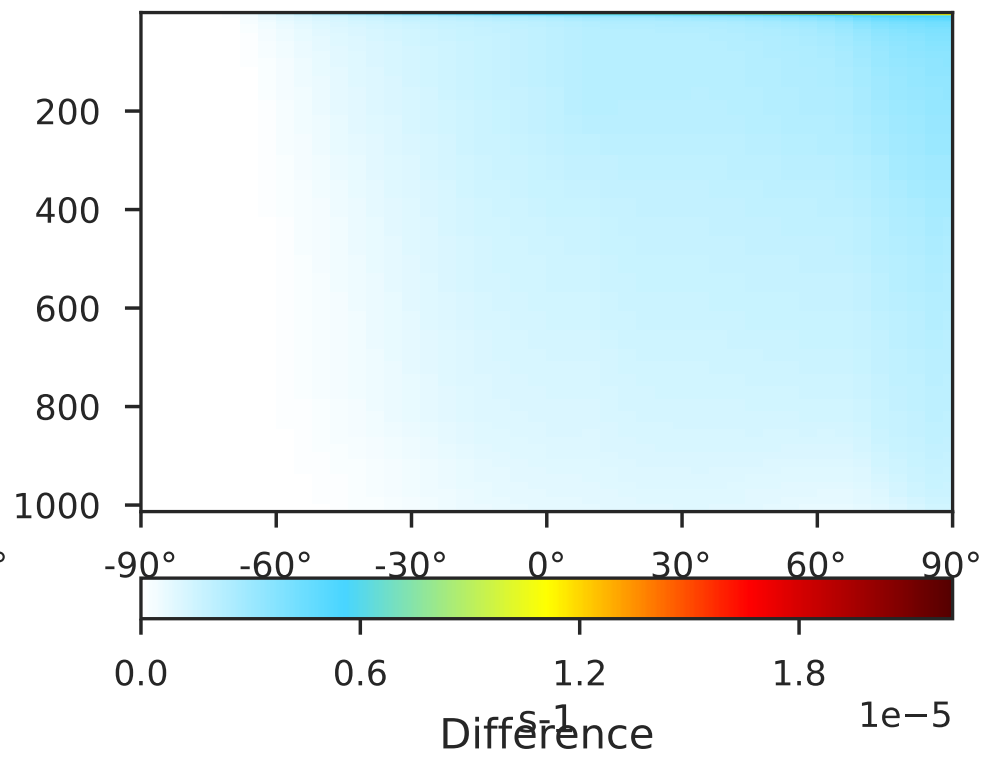
gcc-4x5-1Mon-14.2.0-alpha.20 (Dev) 4.0x5.0
