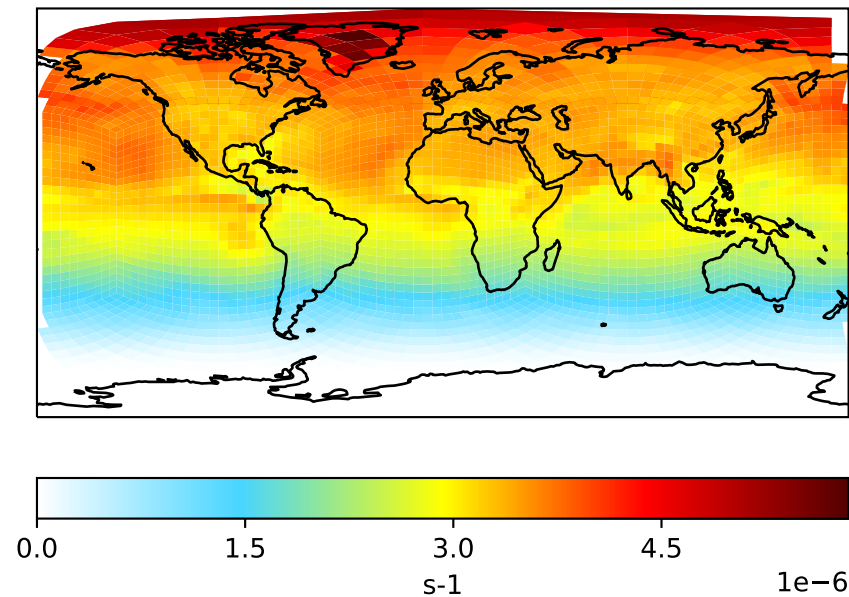
GCHP_dev (Dev) c24
