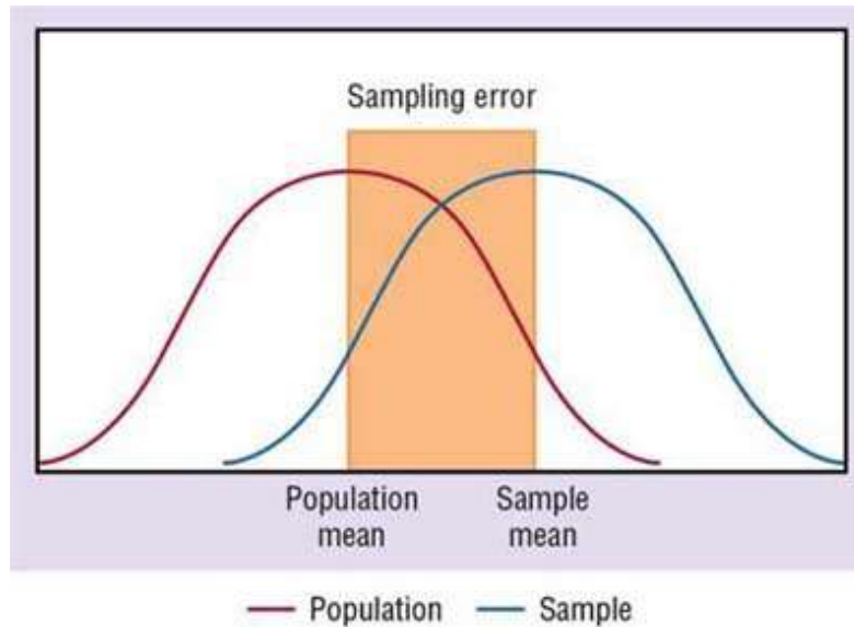
FIG. 15.3 Sampling error.
