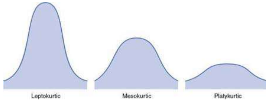
FIG. 21.6 Kurtosis.
