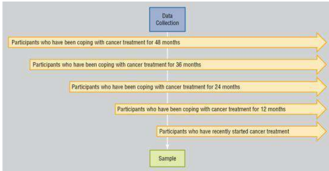
FIG. 10.4 Cross-sectional design.
