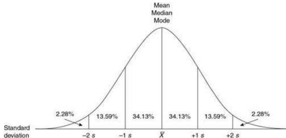
FIG. 21.2 Normal curve.
