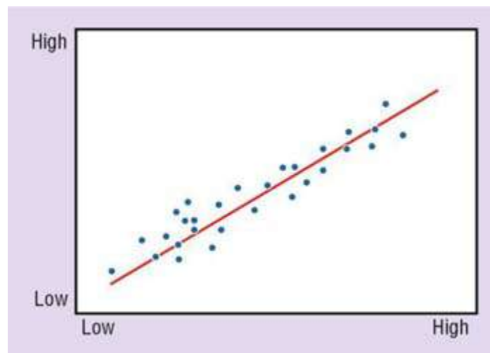
FIG. 8.6 Linear relationship.
