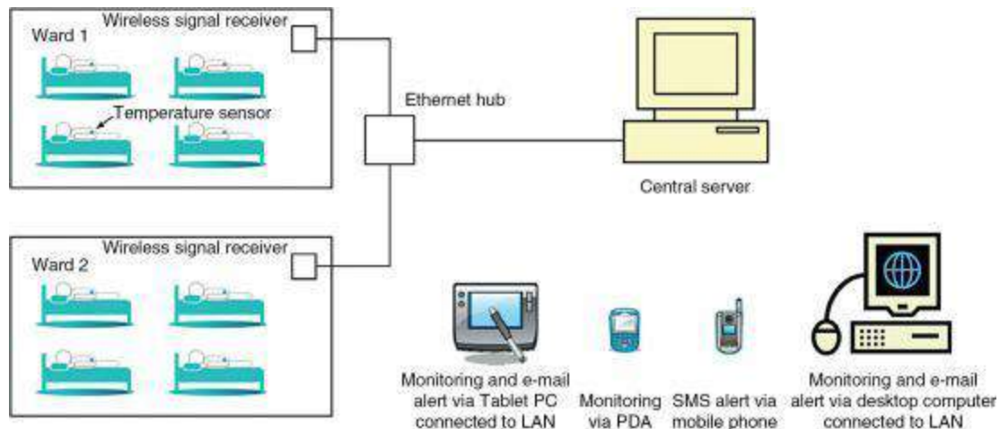
FIG. 17.3 Setup of the ThermoSENSOR wireless temperature monitoring system. Each sensor transmits data wirelessly to a signal receiver (node) that is within the prescribed transmission range. The signal receiver uploads the data to a central server through the local area network (LAN) through which the data can be accessed from computers and other devices that are connected, wirelessly or by wired means, to the LAN. The server can be configured to send out e-mail and short message service (SMS) alerts. Source: (From Ng, K., Wong, S., Lim, S., & Goh, Z. [2010]. Evaluation of the Cadi ThermoSENSOR wireless skin-contact thermometer against ear and axillary temperatures in children. Journal of Pediatric Nursing , 25[3], 177.)
