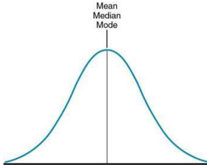
FIG. 21.3 Symmetrical curve.
