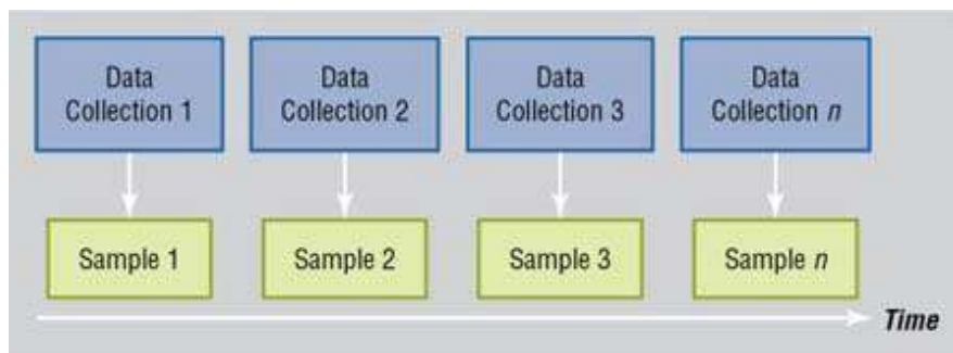
FIG. 10.3 Trend design.
