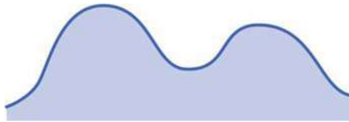
FIG. 21.5 Bimodal distribution.
