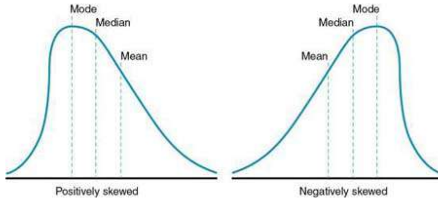
FIG. 21.4 Skewness.
