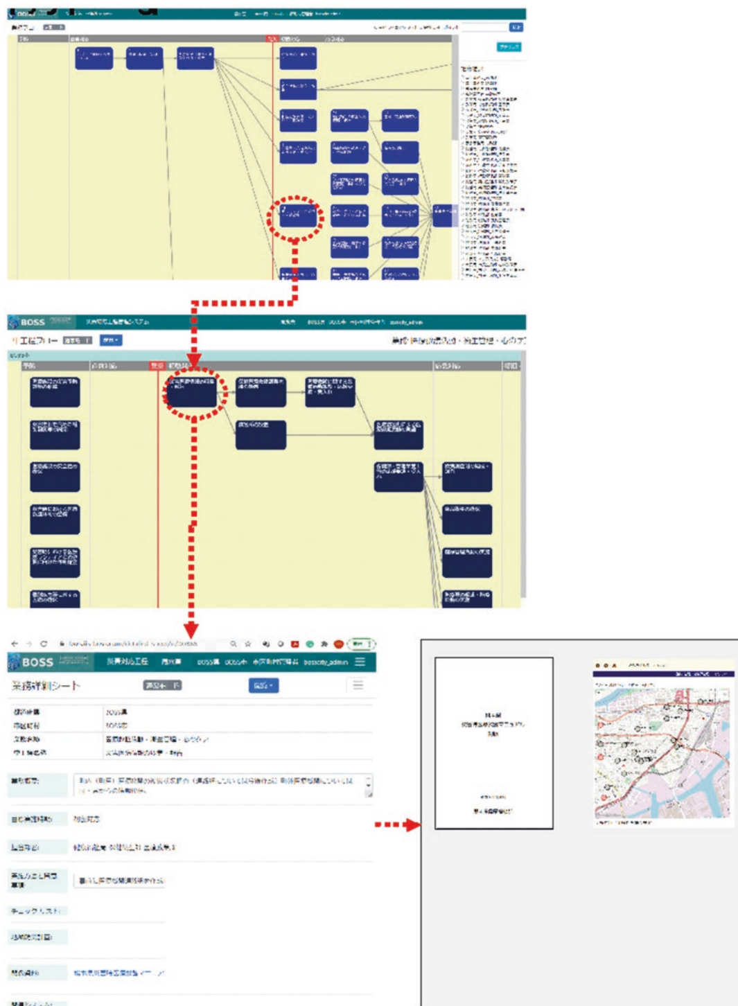
Fig. 21.1 BOSS overview
