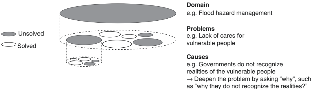
Fig. 27.1 Structuring problems
