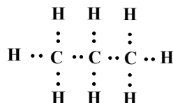
propana
