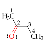
2-butanon
