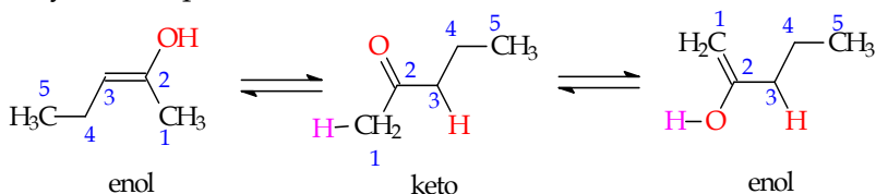
Gambar 10.80 Tautomer keto-enol
