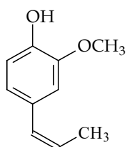
eugenol
