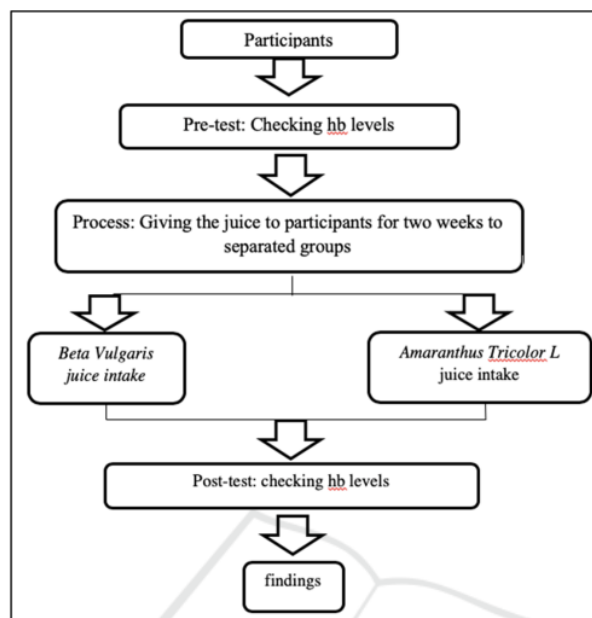
Figure 1: Research flow.
