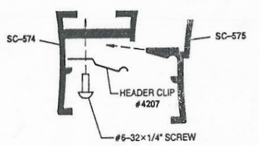
2 - PIECE HEADER DETAIL
