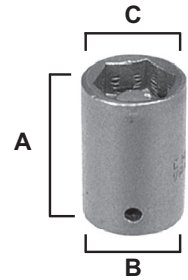
1/4" SQUARE DRIVE
