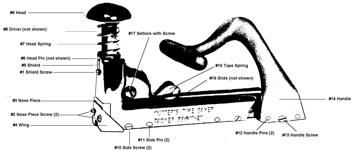
Parts List - Reliable BS#18-20G Tacker
