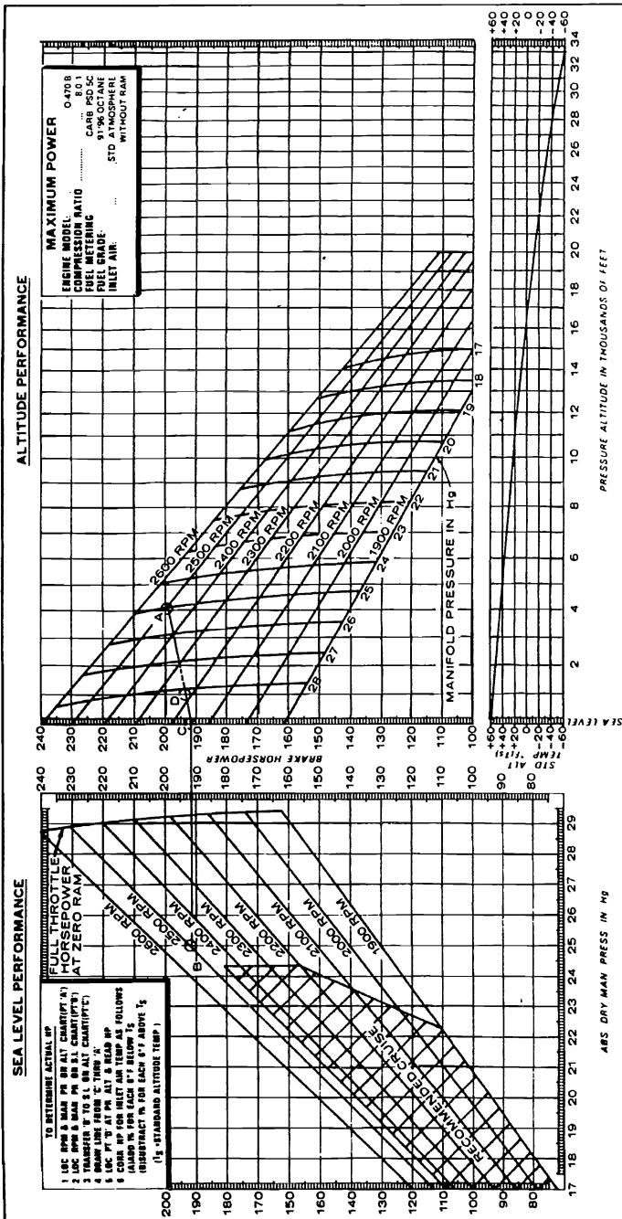
Figure 4. ALTITUDE PERFORMANCE FOR O-470-B
