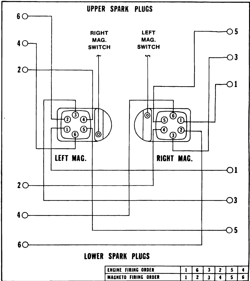
Figure 24. WIRING DIAGRAM
