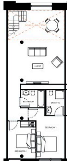
Floor 7
